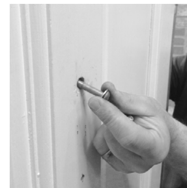
4. Holding key safe, locate fixing through the hole and tighten
